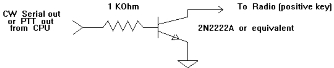
Circuit A: Use this for serial port CW and PTT
